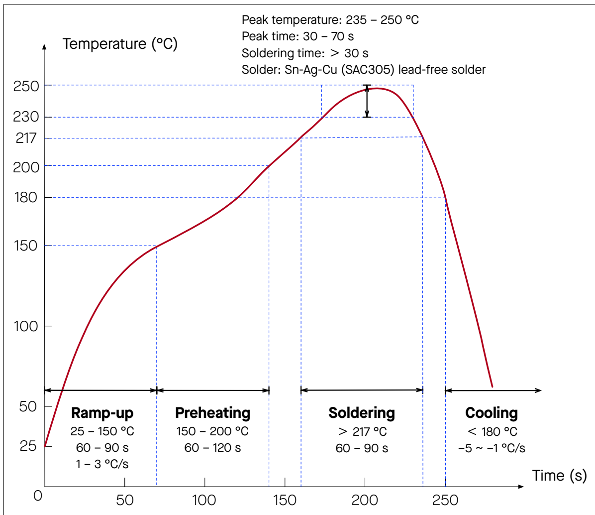
Figure 12-1. Reflow Profile
